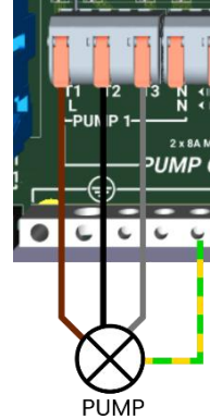
Three-Phase Delta Pump
