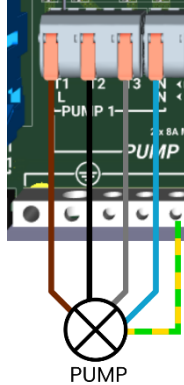
Three-Phase Star Pump
