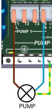
Single-Phase Pump
